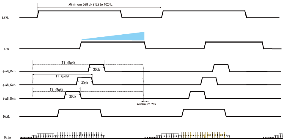
Fig. 11 Shutter-Select mode with internal line rate generator (and individual exposure)
