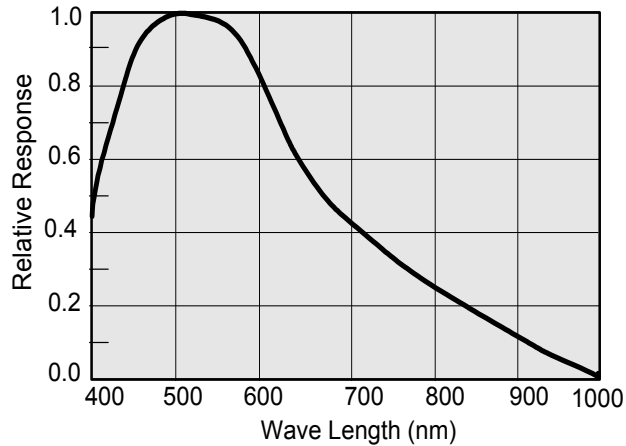
Fig. 30. Spectral sensitivity.
