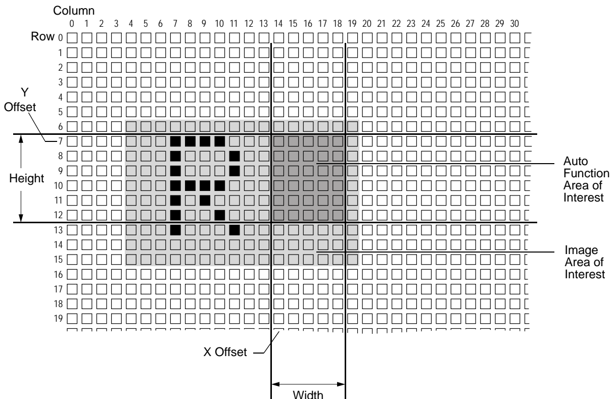
Fig. 41: Auto Function Area of Interest and Image Area of Interest
