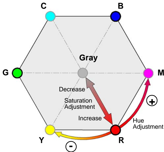
Fig. 37: Hue and Saturation Adjustment In the Color Hexagon. Adjustments Are Indicated for Red as an Example
