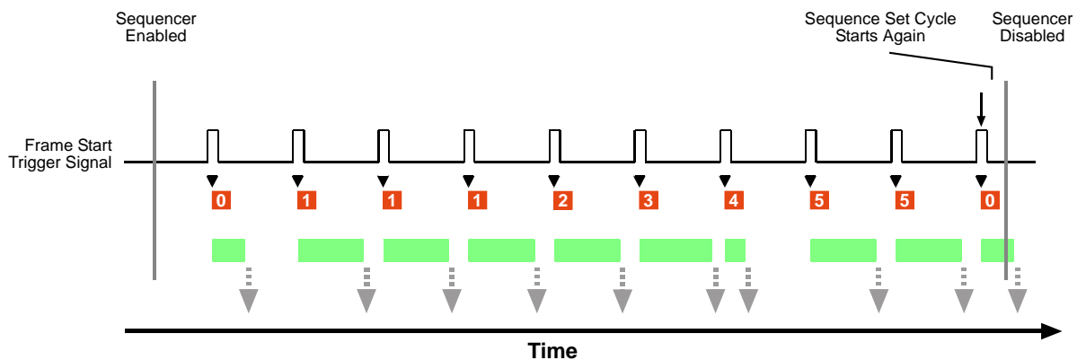
Fig. 45: Sequencer in Auto Sequence Advance Mode
