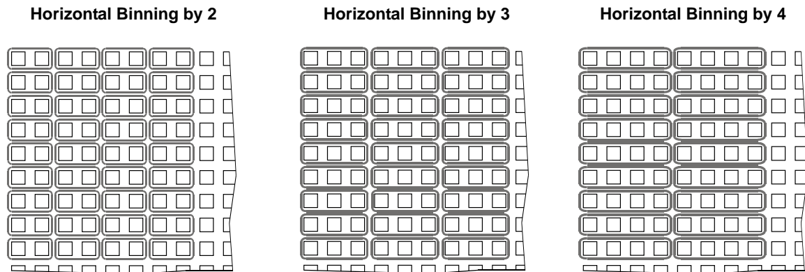
Fig. 53: Horizontal Binning
