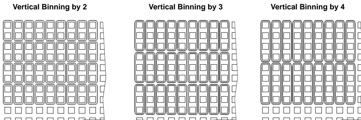
Fig. 52: Vertical Binning
