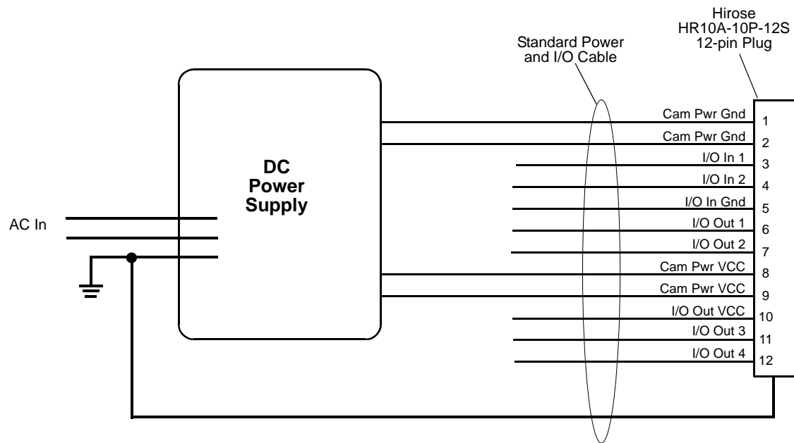
Fig. 11: Standard Power and I/O Cable
