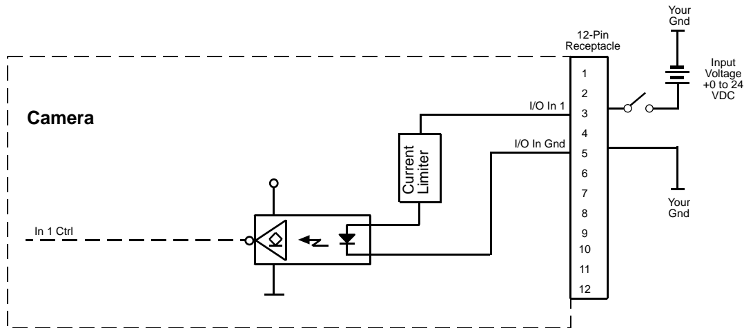
Fig. 12: Typical Input Circuit (Simplified)
