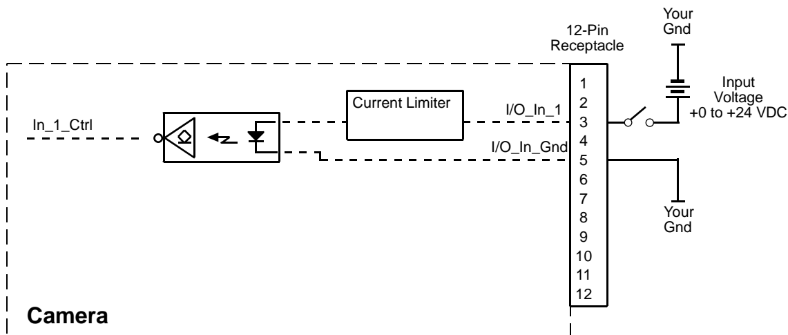
Fig. 38: Typical Voltage Input Circuit
